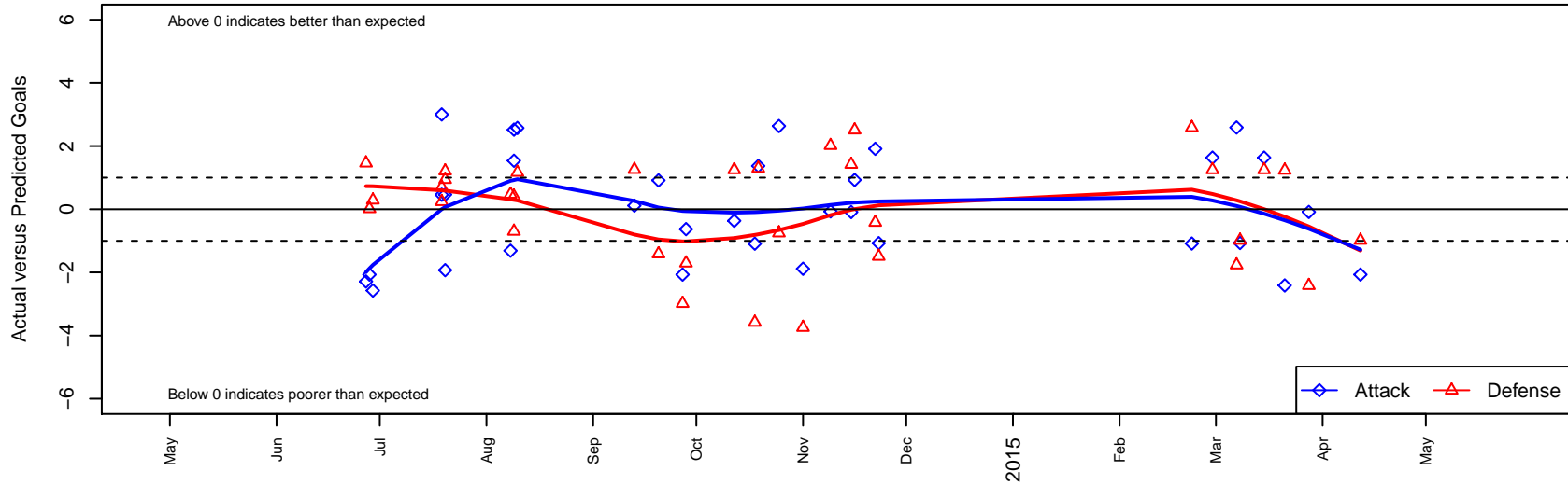
Tynecastle FC B03 Dots are actual minus expected GF (blue circles) and GA (red triangles). Blue line is smoothed change in attack strength. Red is smoothed change in defense strength.
